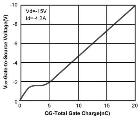
Figure 5: Gate-Charge Characteristics
