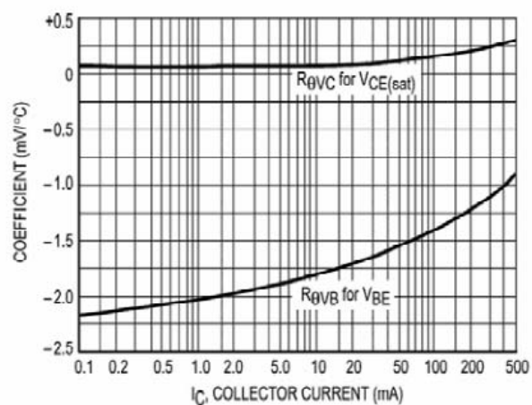
Temperature Coefficients
