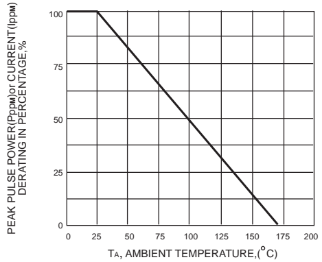
FIG. 2-PULSE DERATING CURVE
