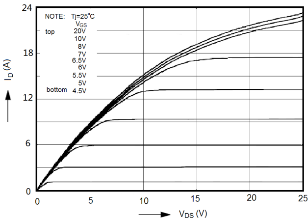
Figure3. Output characteristics
