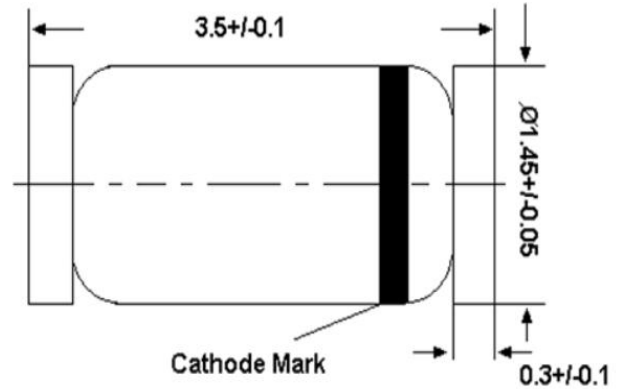
Glass case MiniMELF Dimensions in mm
