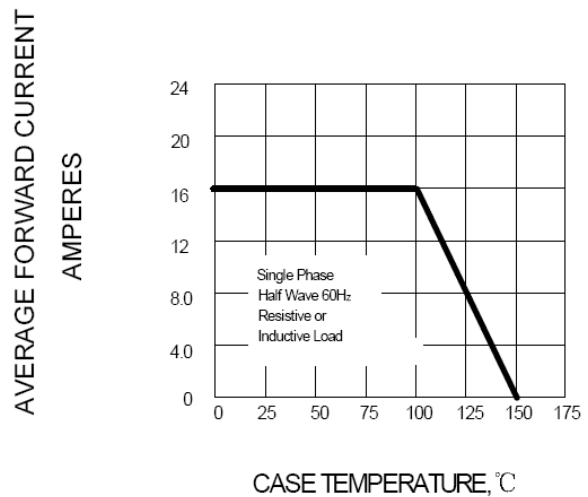
FIG.4-FORWARD DERATING CURVE
