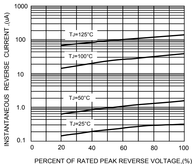
FIG.5-TYPICAL REVERSE CHARACTERISTICS
