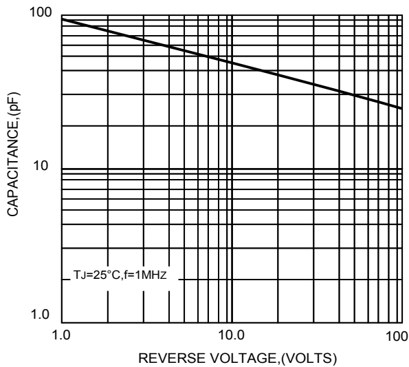
FIG.3-TYPICAL JUNCTION CAPACITANCE
