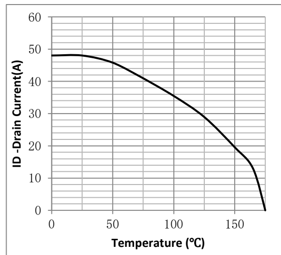
Fig.12 ID vs. Junction Temperature ③
