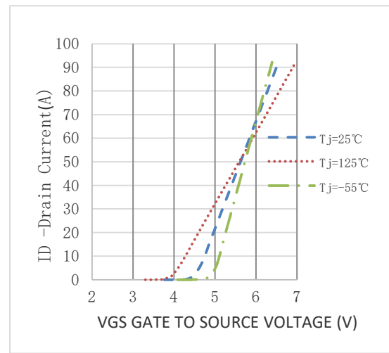
Figure 10. Transfer Characteristics
