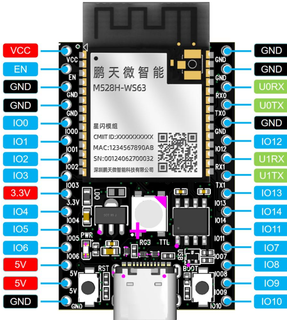
E528H-WS63管脚定义
