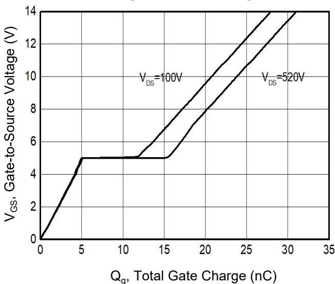
Figure 5. Gate Charge
