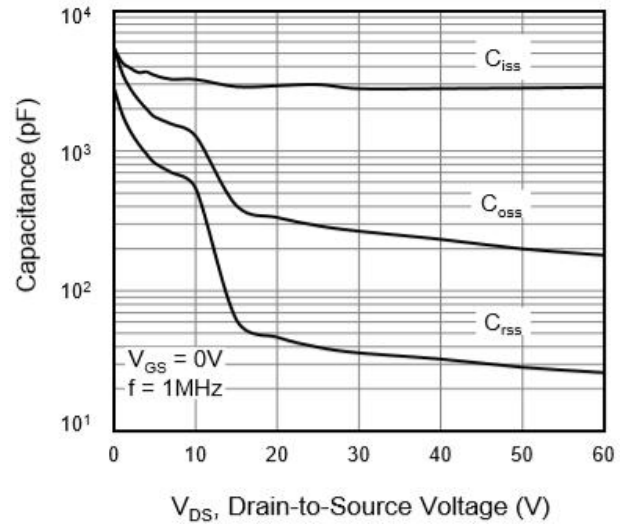
Figure 8. Capacitance
