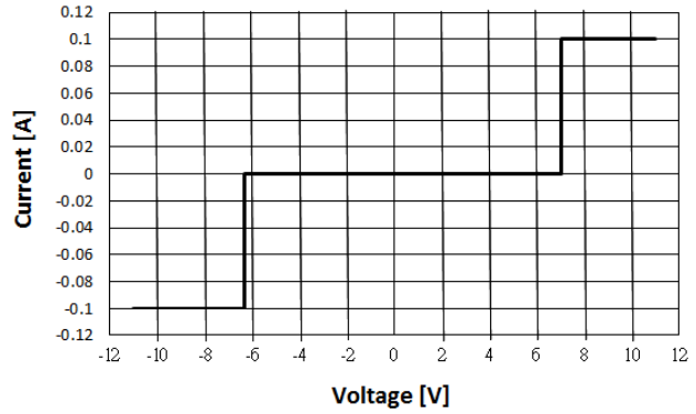
Voltage Sweeping of I/O_1 to I/O_2
