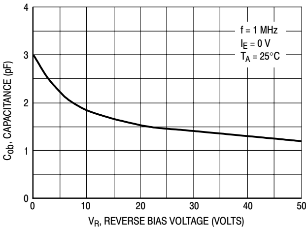
Figure 14. Output Capacitance
