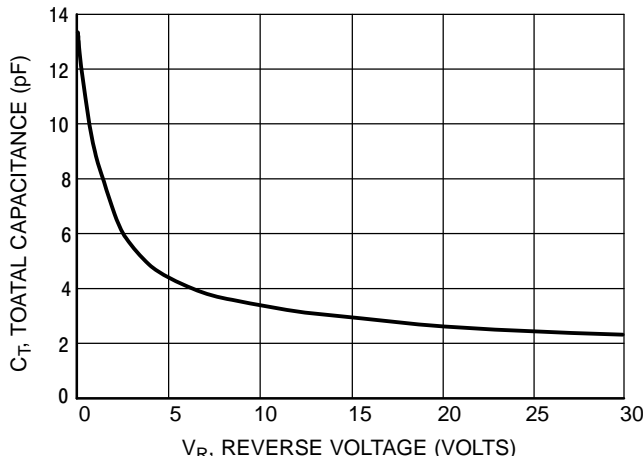
Figure 4. Total Capacitance
