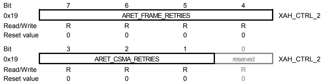
Figure 7-21. Register XAH_CTRL_2.
