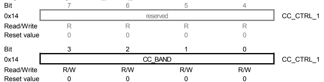
Figure 9-20. Register CC_CTRL_1.
