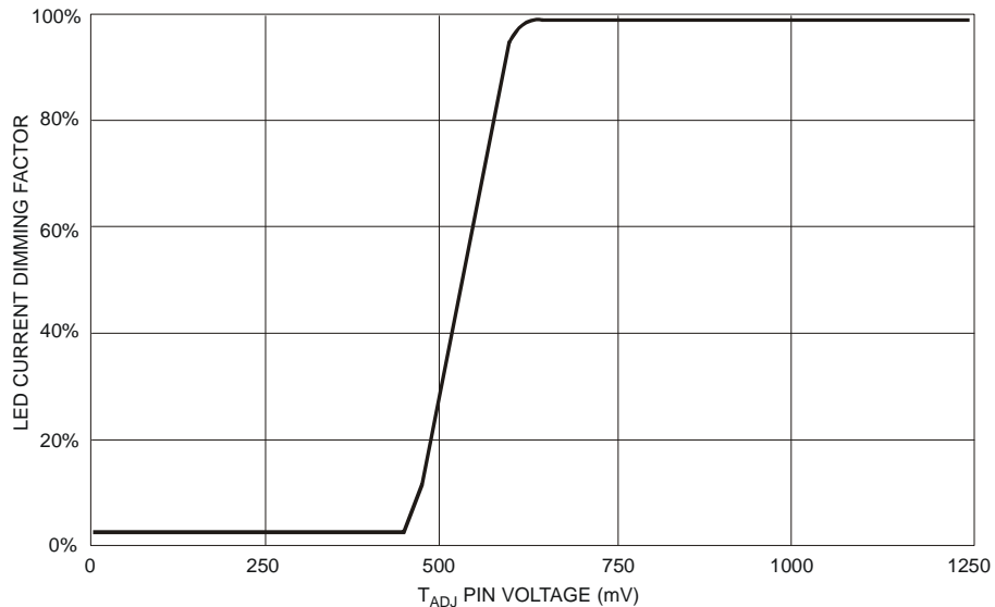
LED Current Dimming Factor vs. T_{ADJ} Voltage
