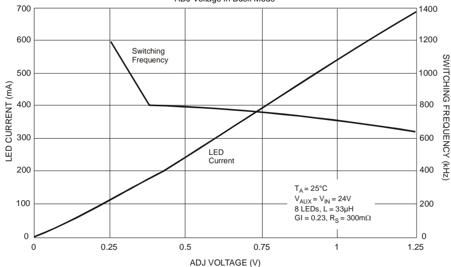
LED Current and Switching Frequency vs. ADJ Voltage in Buck-Boost Mode
