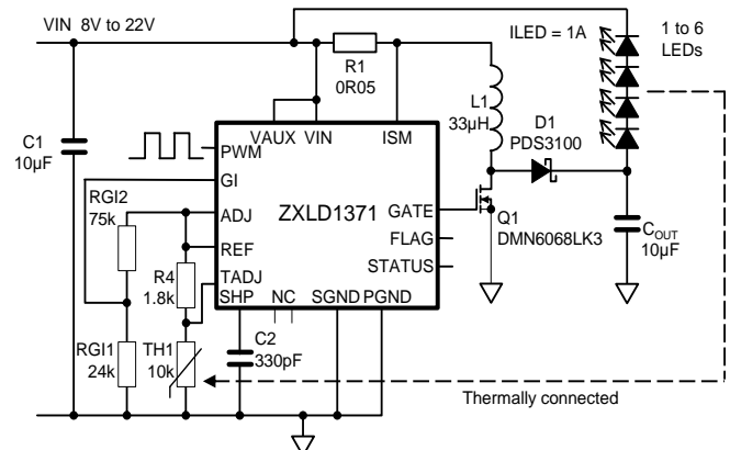
Buck-Boost Diagram Utilizing Thermistor and T ADJ
