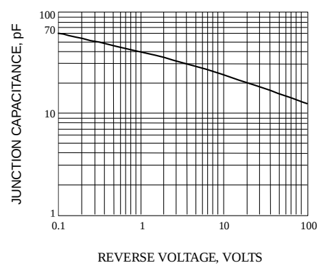
Fig. 6-TYPICAL JUNCTION CAPACITANCE
