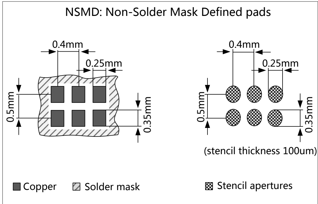
Figure 34. Footprint
