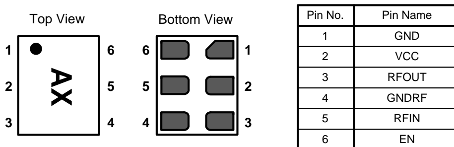
Figure 1. AW5015 Pin Configuration and Marking
