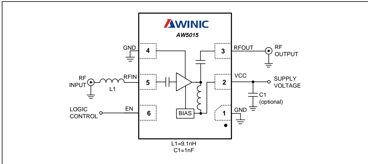
Figure 2. Application Schematic AW5015
