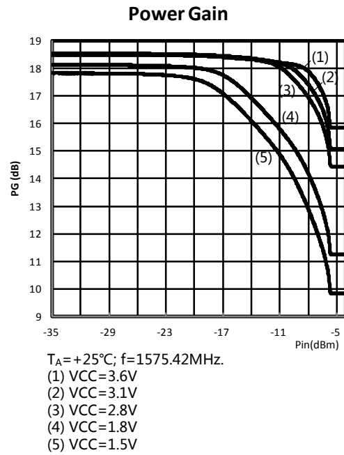
Figure 12. Power Gain as a function of input power; typical values
