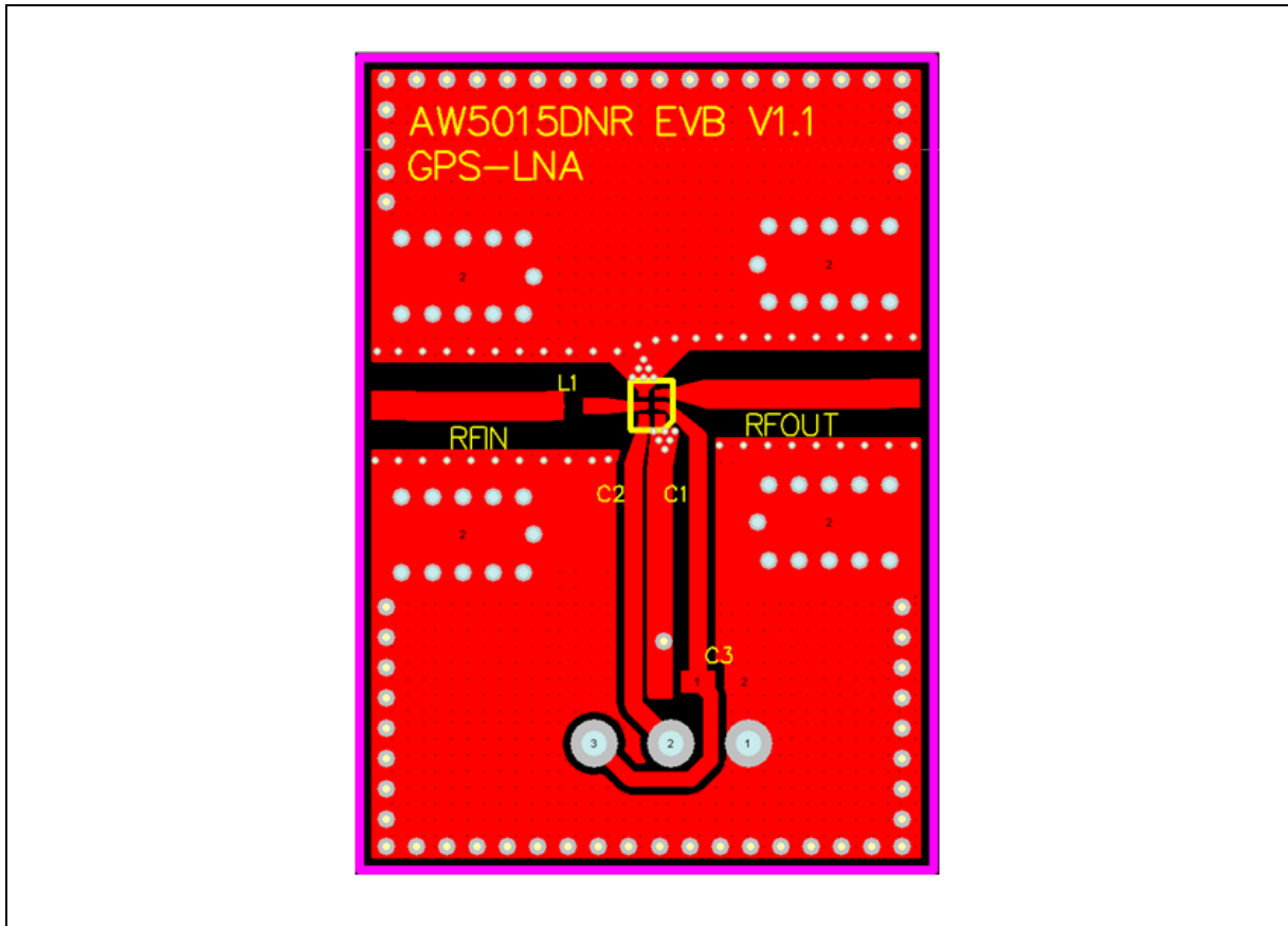
Figure 26. Drawing of Application Board
