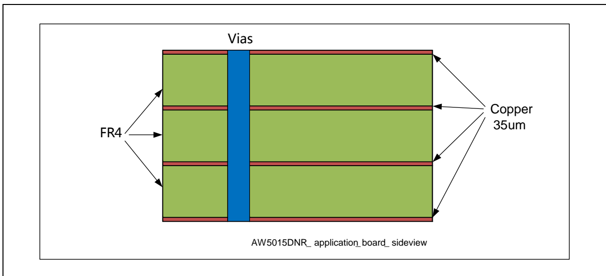
Figure 27. Application Board Cross-Section
