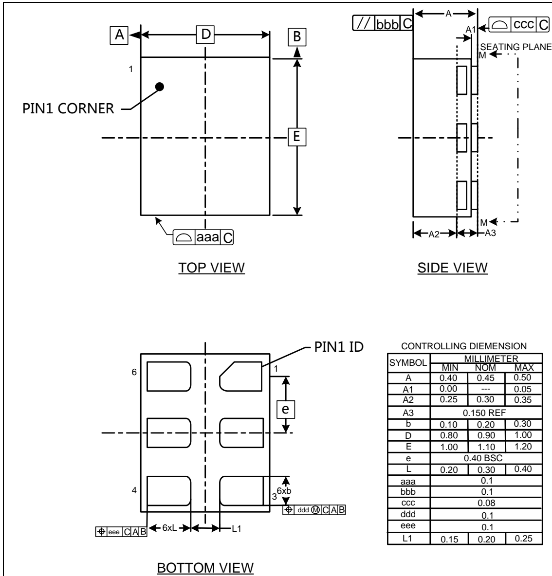
Figure 32. Package Outline
