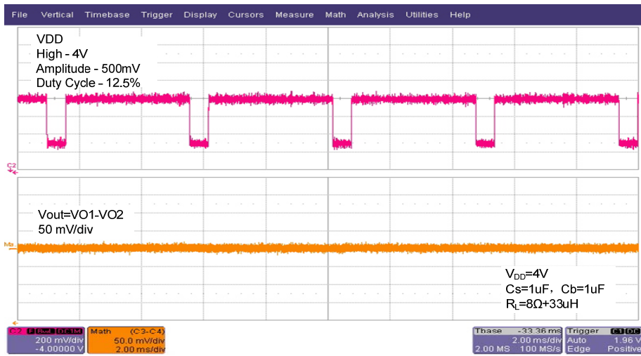
图 6 GSM POWER SUPPLY REJECTION vs TIME
