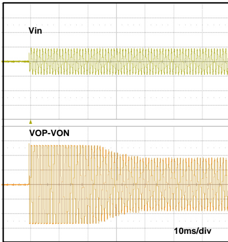
SINGLE-LEVEL-AGC 功能启动时序
