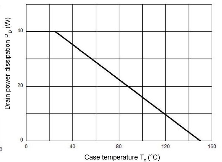
Figure 10.2 Power Dissipation vs. Temperature TO-251/TO-252/TO-263/TO-262
