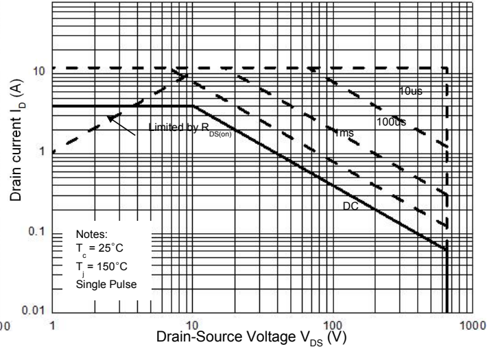
Figure 9.2 Maximum Safe Operating Area TO-251/TO-252/TO-263/TO-262
