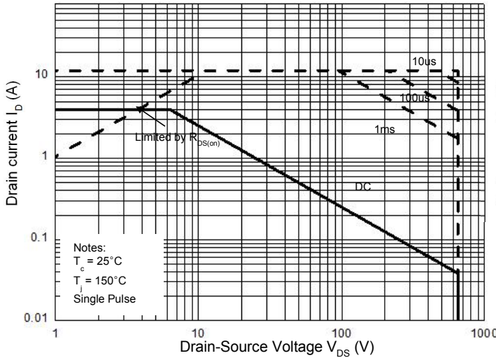
Figure 9.1 Maximum Safe Operating Area TO-220MF
