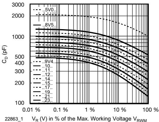
Fig. 3 - Typical Capacitance C_D vs. Reverse Voltage V_R
