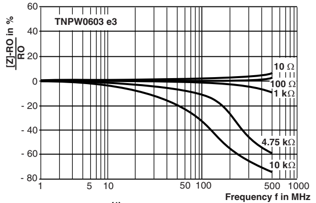
HF Performance (1)
