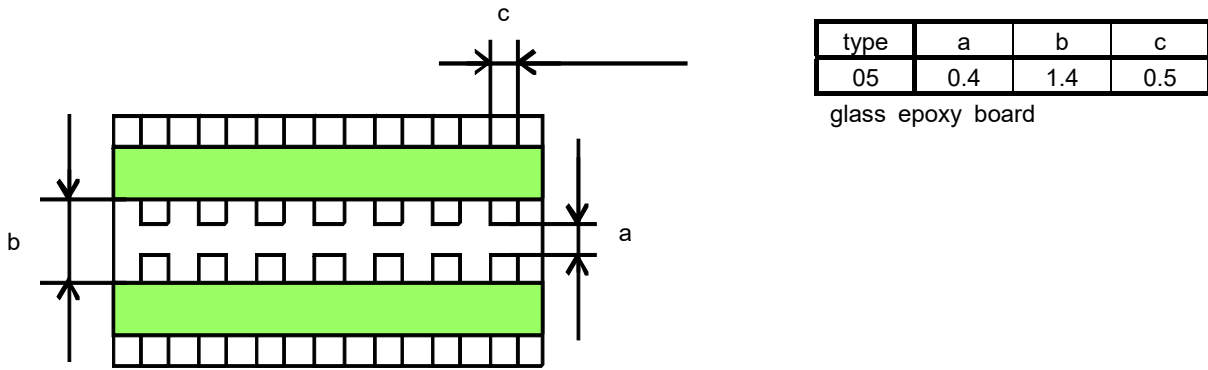
Fig.1 Substrate for temperature cycle test
