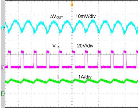
Output Ripple ( V_{IN}=24V, V_{OUT}=5V, I_O=1A )
