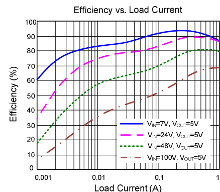
Figure 2. Efficiency
