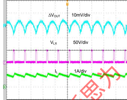
Output Ripple ( V_{IN}=48V, V_{OUT}=5V, I_O=1A )
