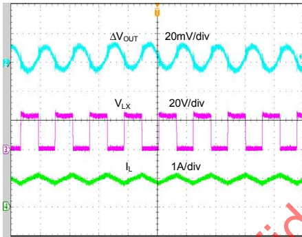
Output Ripple ( V_{IN}=24V, V_{OUT}=12V, I_O=1A )
