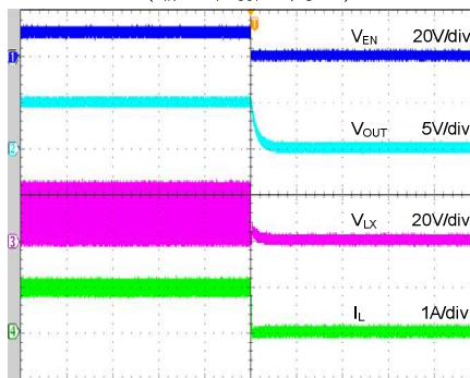
Time (400μs/div)
