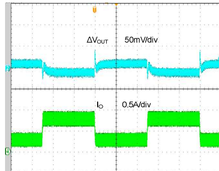
Load Transient ( V_{IN}=48V, V_{OUT}=5V, I_O=0.25 \sim 0.75A )
