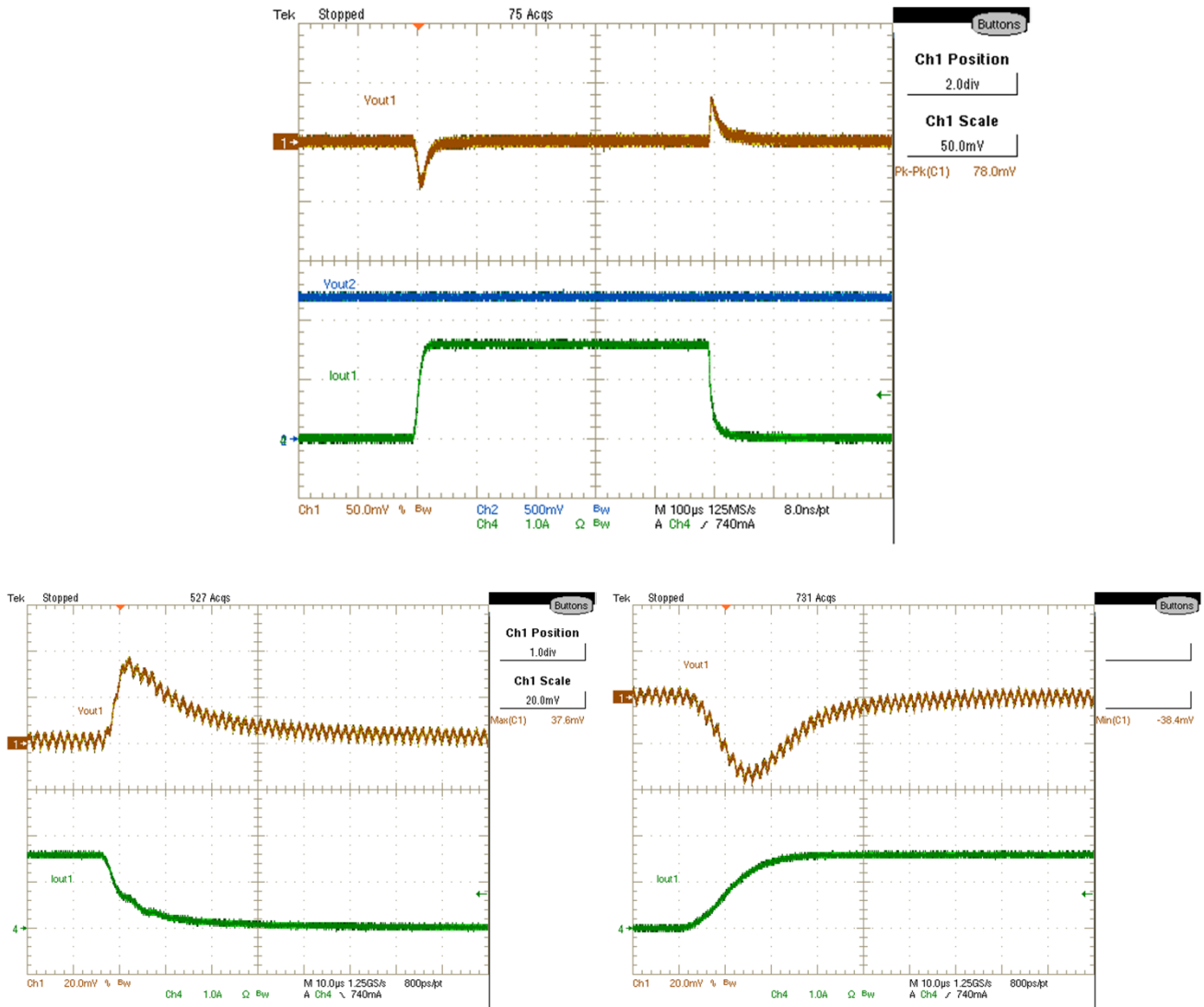
Fig. 15: Transient Response of channel1 0A-1.6A (0-40%), Ch 1 :Vout 1 , Ch 2 :Vout 2 , Ch 4 : Iout 1
