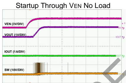
Time-1ms/div
