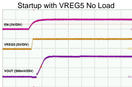
Time-1ms/div
