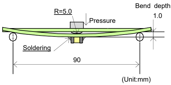
Fig.3 Testing status
