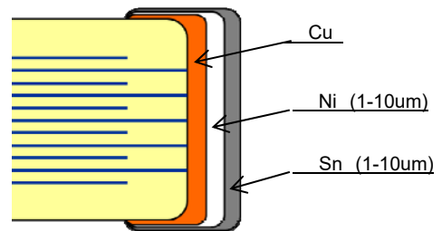
Fig. Internal structure
