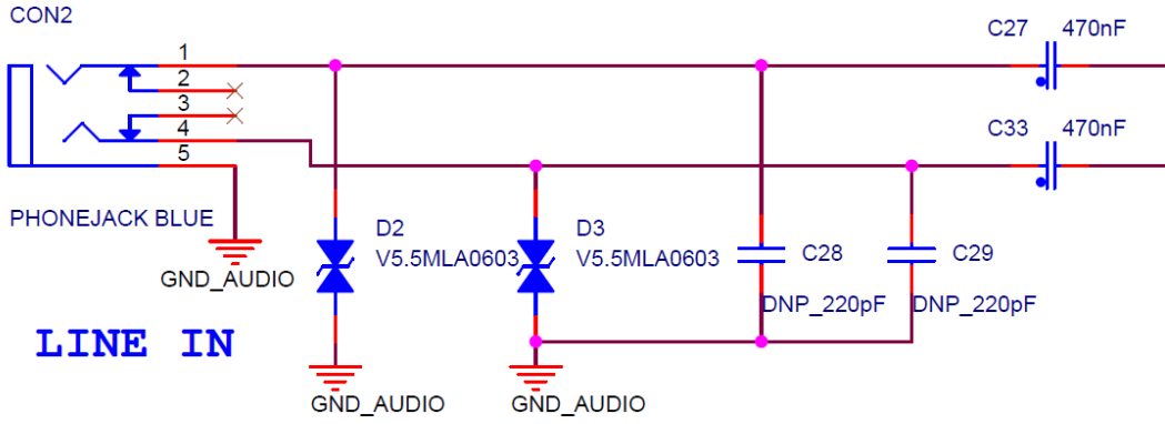
图 6 LINE IN
