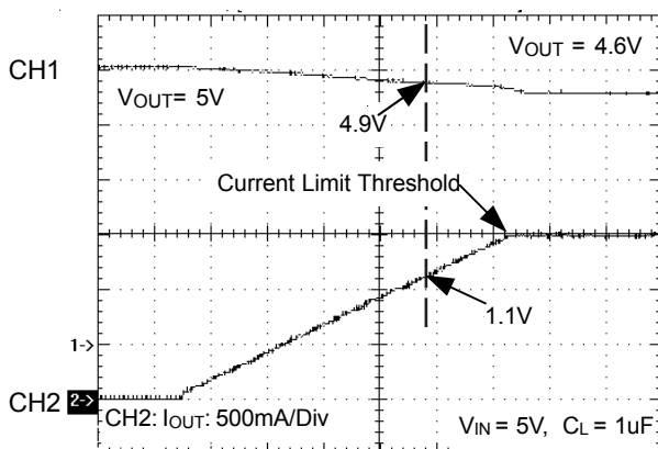
Ramped Load Response
