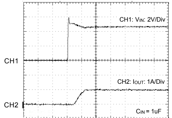
Soft - start Short Circuit Response
