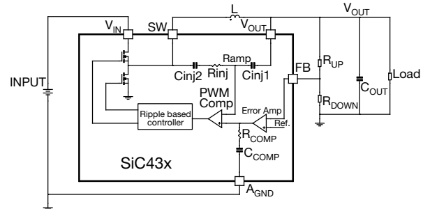
Fig. 5 - VM-COT Block Diagram
