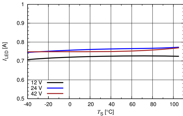
I_{LED} versus T_S ( R_{sense} = 158\text{ m}\Omega , L = 68\text{ }\mu\text{H} )
