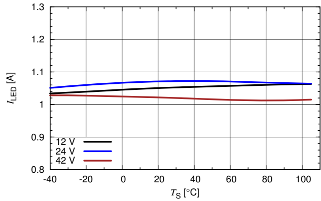
I_{LED} versus T_S ( R_{sense} = 110\text{ m}\Omega , L = 68\text{ }\mu\text{H} )
