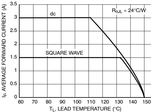
Figure 5. Current Derating - Junction to Lead
