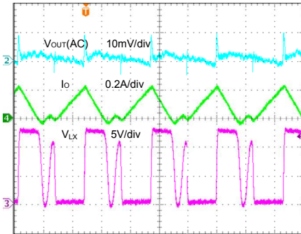
Output Ripple ( V_{IN}=5.0V , V_{OUT}=12V , I_{OUT}=20mA )
