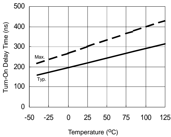
Figure 4A. Turn-On Time vs. Temperature
