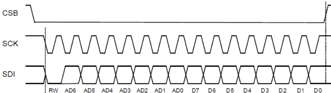
Figure 8: 3-wire SPI read and write sequence
