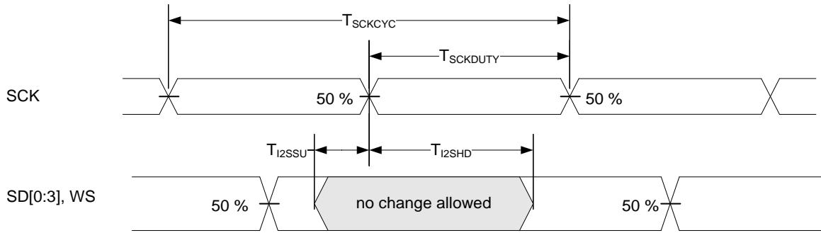
Figure 4.4. I 2 S Input Timing
