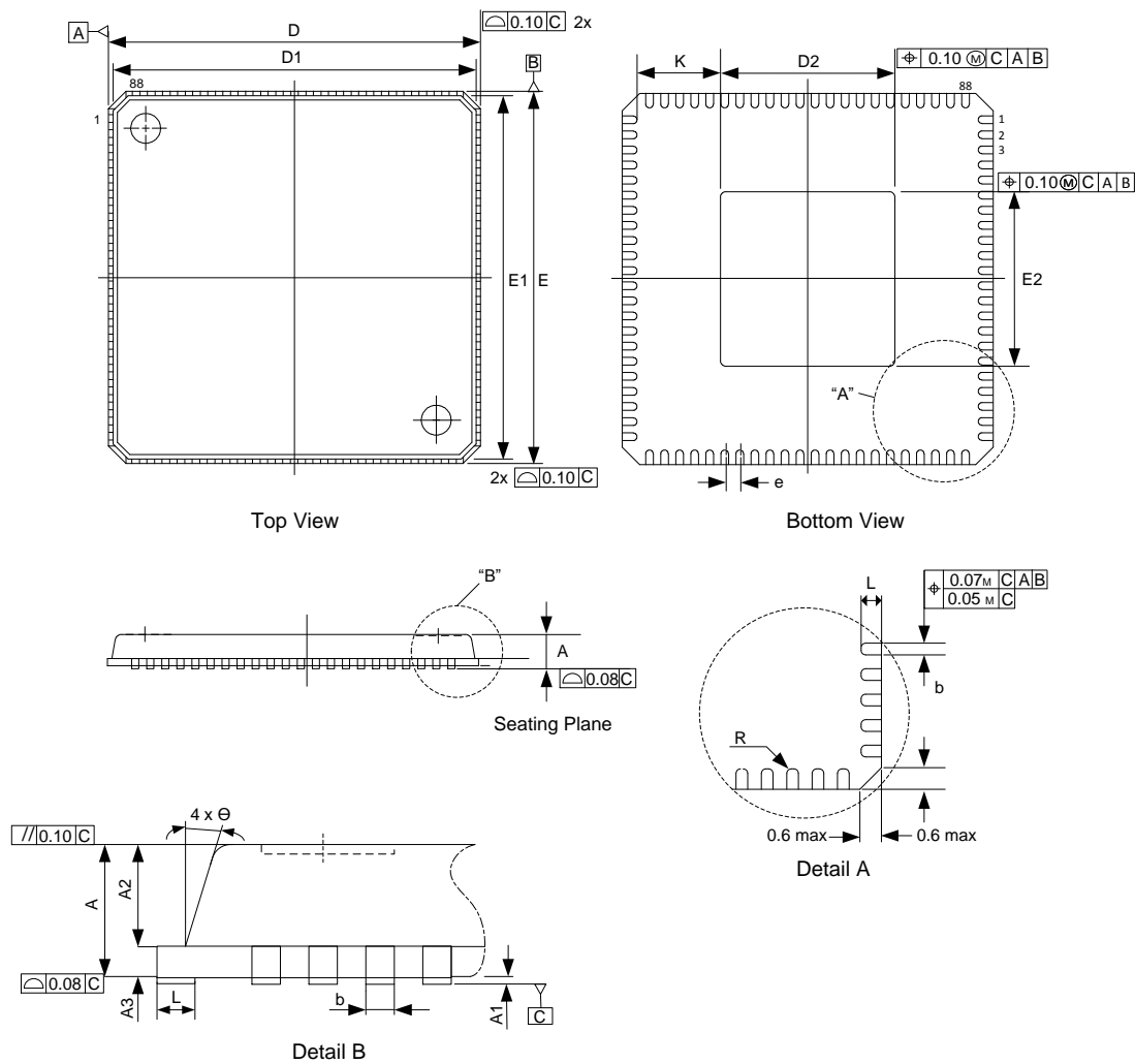
Figure 8.1. Package Diagram
