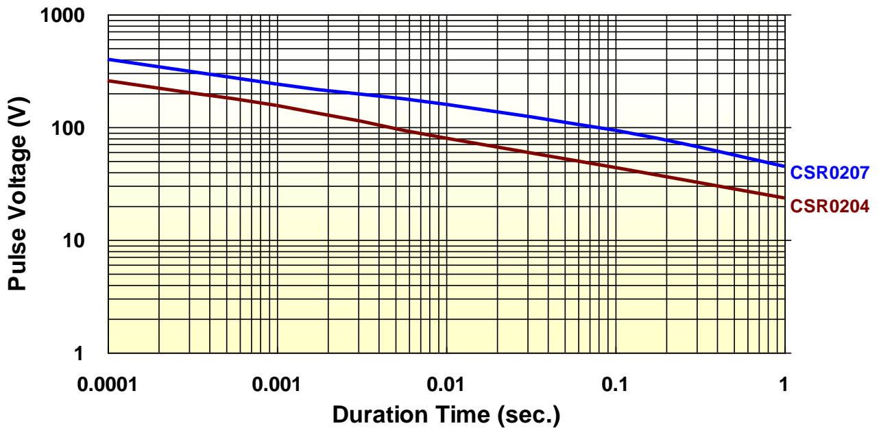
CSR Series Pulse Voltage(100 Ohm)
