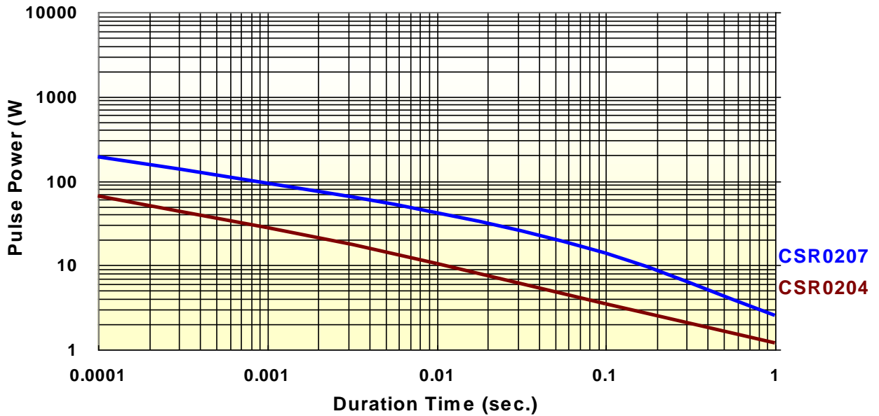
CSR Series Continuous Pulse(100 Ohm)
