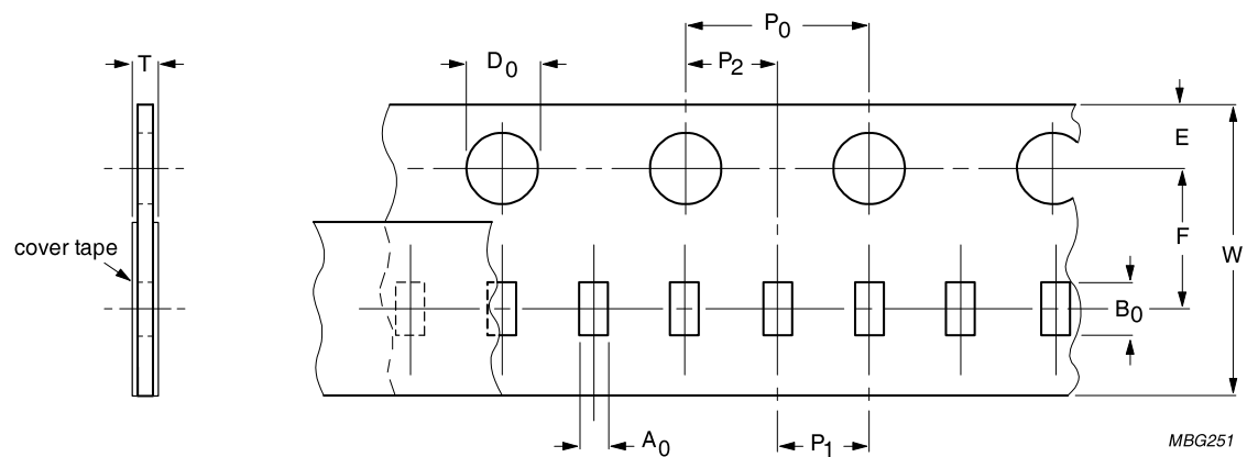
Fig. 4 Paper Tape
