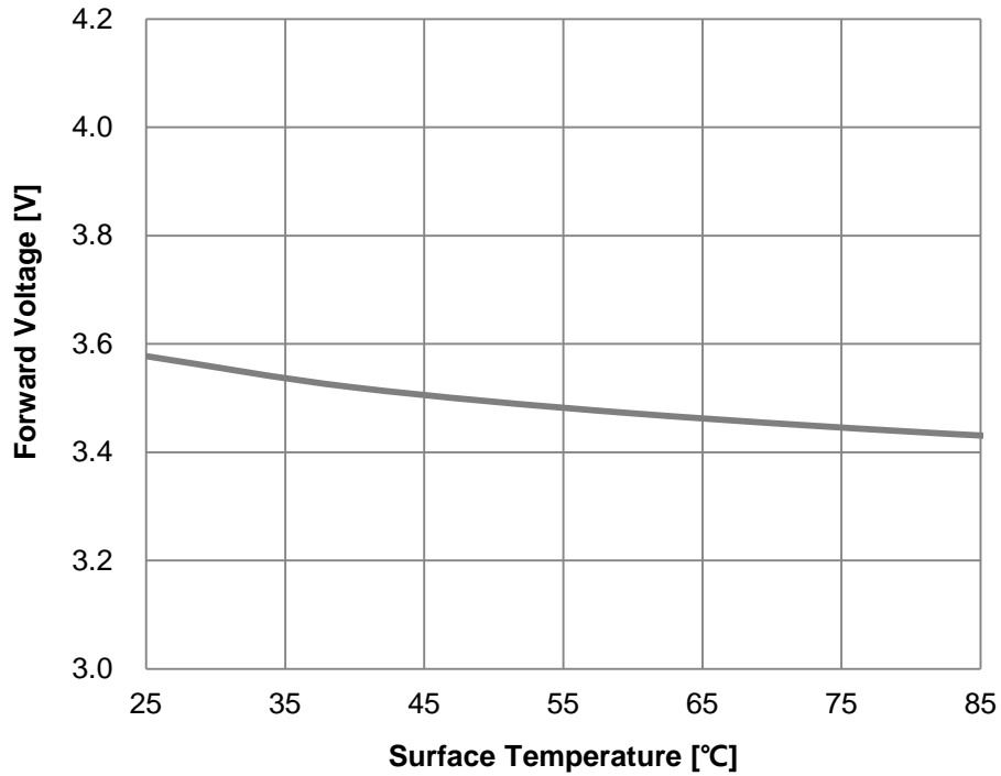
Fig 7. Surface Temperature vs. Forward Voltage, I_F=50\text{mA}
