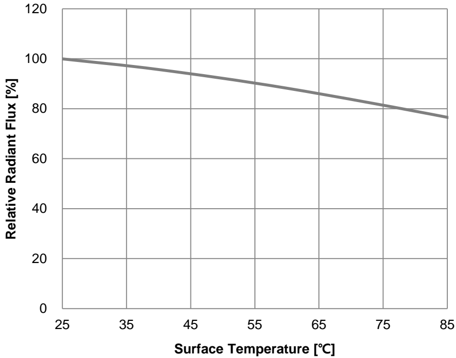
Fig 5. Surface Temperature vs. Relative Radiant Flux, I_F=50\text{mA}
