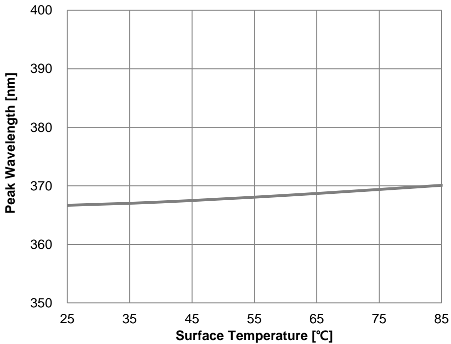
Fig 6. Surface Temperature vs. Peak Wavelength, I_F=50\text{mA}
