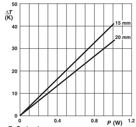
Ø 0.58 mm FeCu-leads Minimum distance from resistor body to PCB = 1 mm PR01 Temperature rise ( \Delta T ) at the lead end (soldering point) as a function of dissipated power at various lead lengths after mounting.
