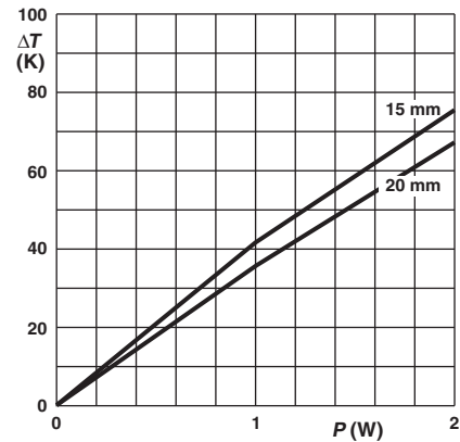
Ø 0.78 mm Cu-leads Minimum distance from resistor body to PCB = 1 mm PR02 Temperature rise ( \Delta T ) at the lead end (soldering point) as a function of dissipated power at various lead lengths after mounting.
