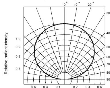
Fig.6 Radiation diagram
