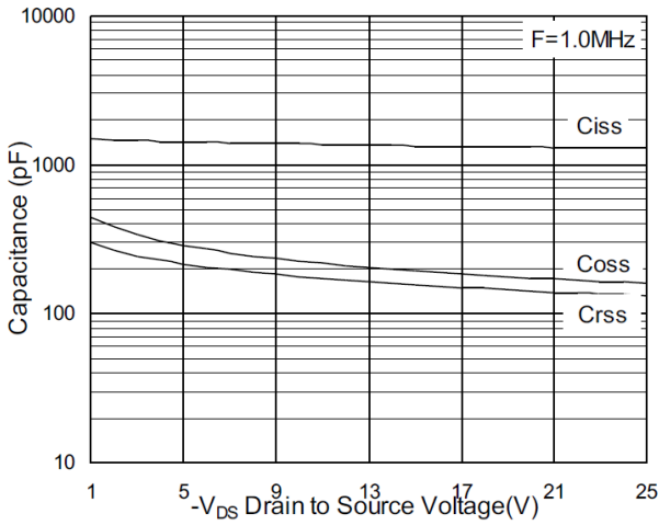
Figure 7 Capacitance Characteristic
