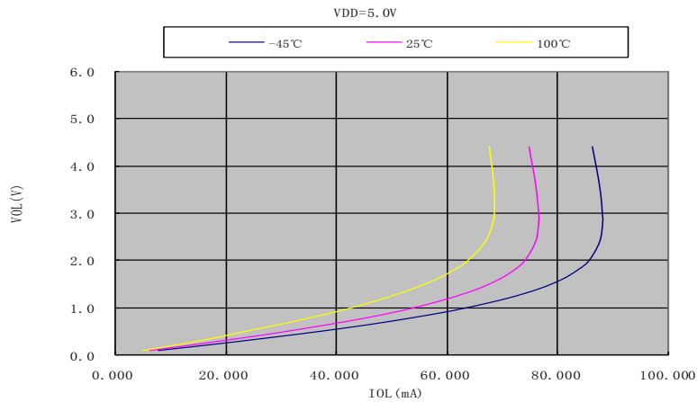
D: V_{OL} vs I_{OL} @ V_{DD}=5.0V
