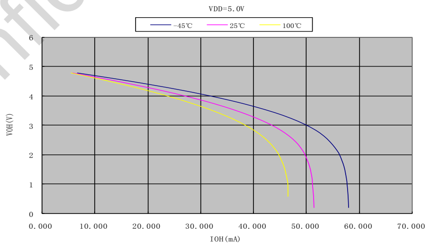
C: V_{OH} vs I_{OH} @VDD=5.0V
