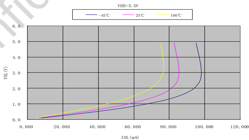
F: V_{OL} vs I_{OL} @ V_{DD}=5.5V
