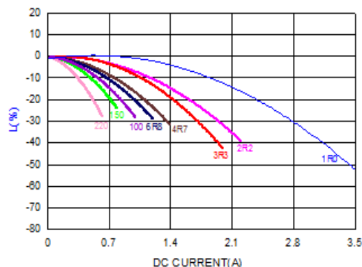
HXNR4012B-SERIES
