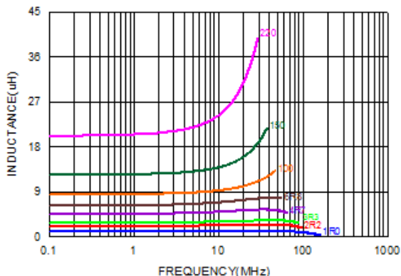
HXNR4012B-SERIES
