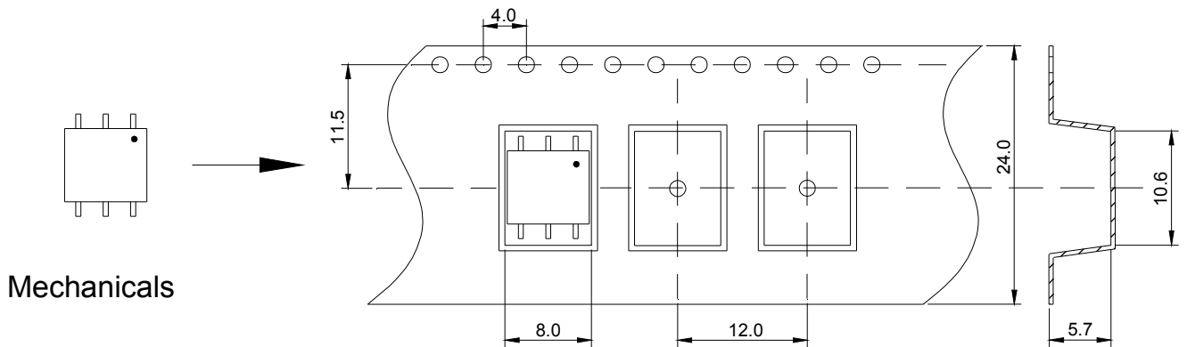
Tape & Reel
