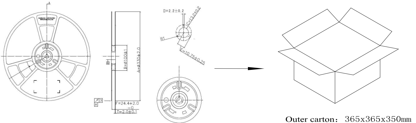
Tape & Reel
