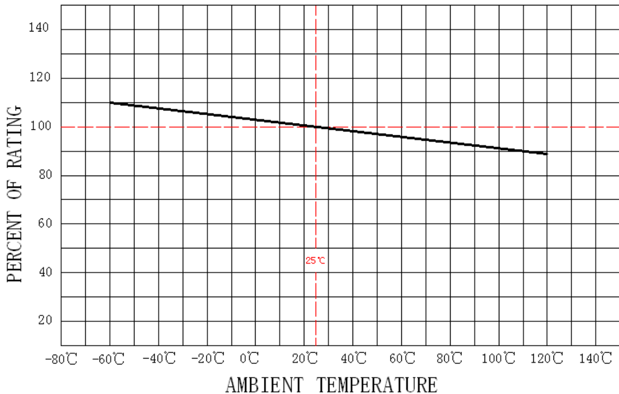
Temperature-Current curve:
