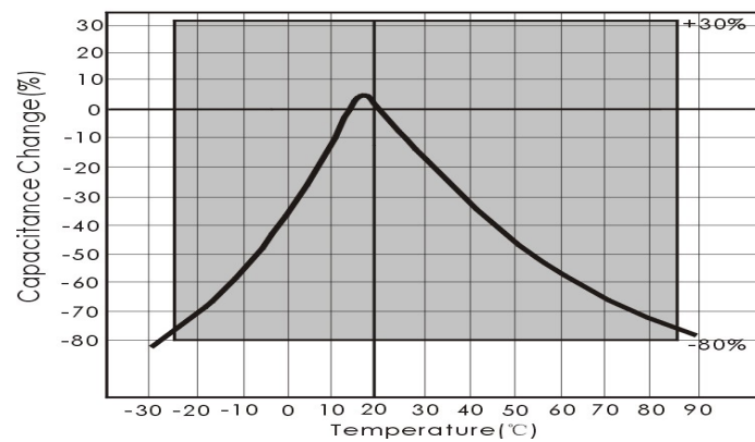
Char:F (Y5V)
