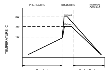
Figure 3. Hand Soldering
