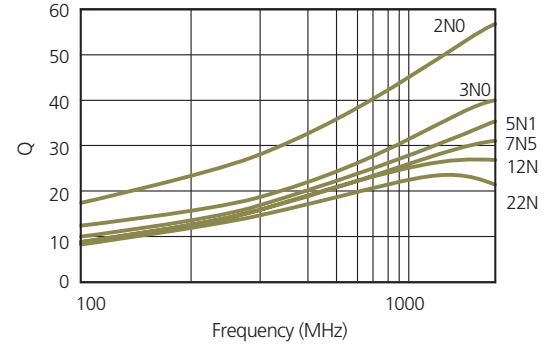
Q CHARACTERISTIC
