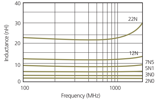
INDUCTANCE
